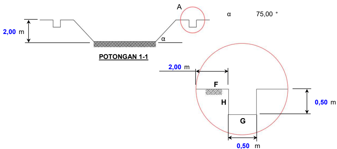
DETAIL A
